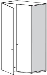
ANBAUELEMENT B 100 1.330,- H 234 cm / IH 226.8 cm B 100 cm / IB 97.5 cm T 62.2 cm / IT 57.3 cm Leistengriff 90° / T 1.8 cm / coal
